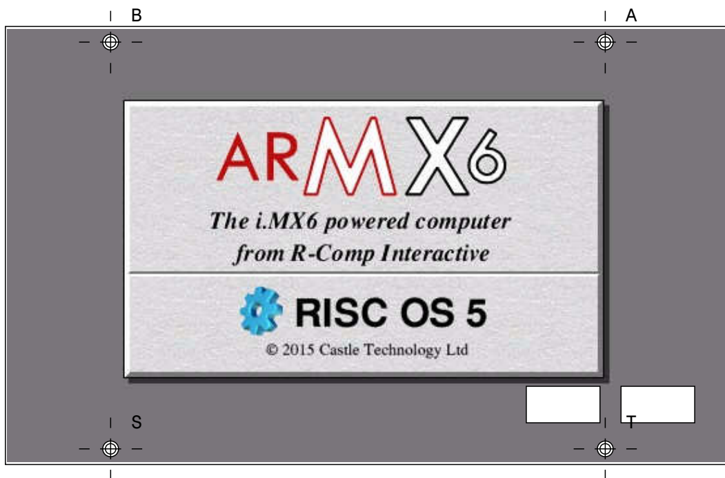
FRONT 84x138x2 Holes ABST 6BA csk Cutout for USB hub
